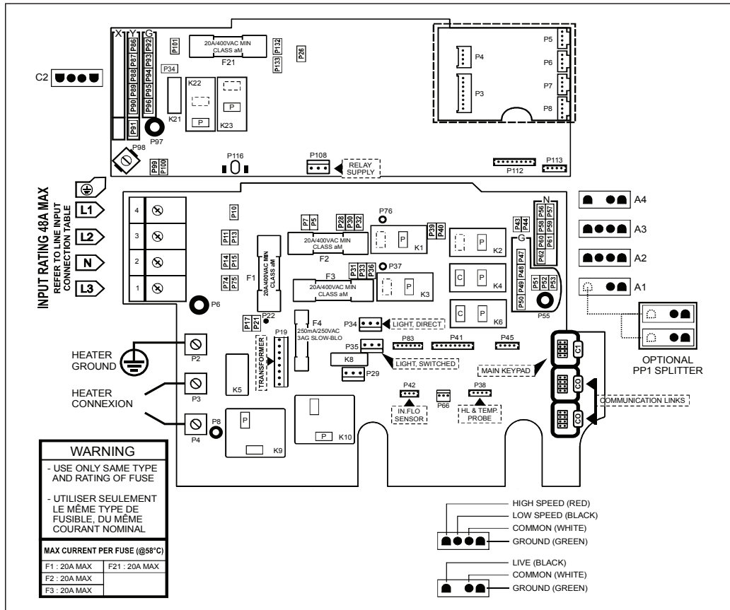
Pump 2 (C2)
