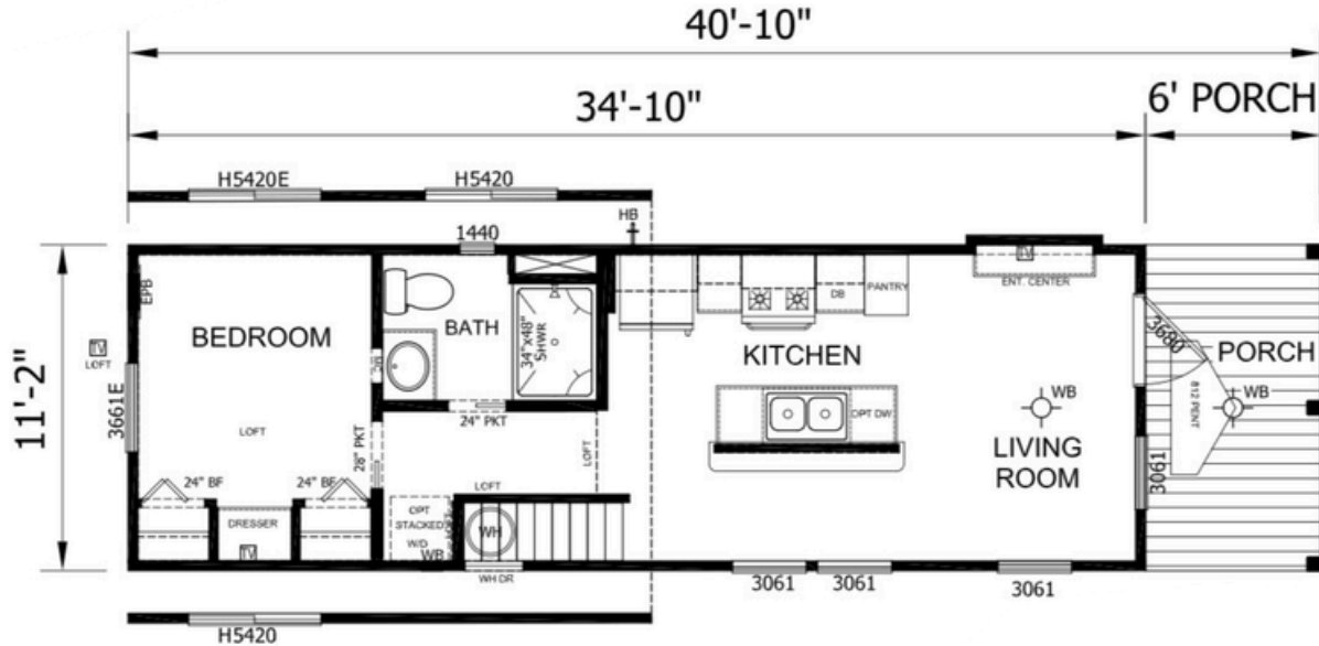
APS-602-SL 1 BEDROOM 1 BATH 11'-2" x 34'-10" 399 SQ. FT. TOTAL
