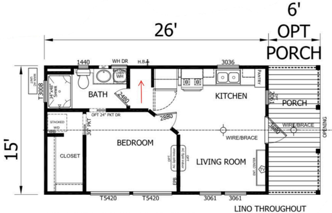
APS-522A WALK IN CLOSET 1 BEDROOM 1 BATH 15'-0" x 26'-0" 399 SQ. FT.
