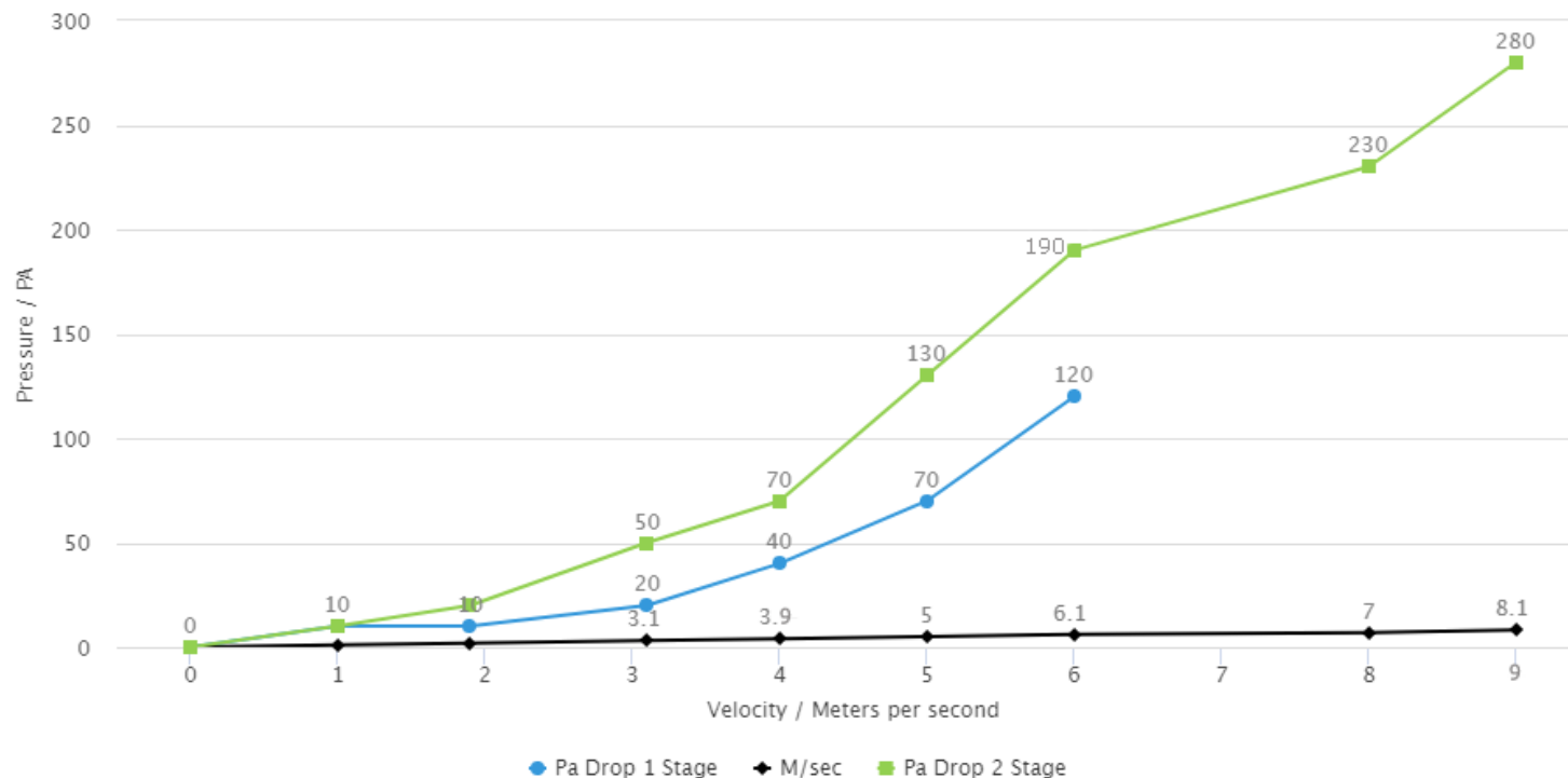
Single Stage & Two Stage Pressure Drop Data
