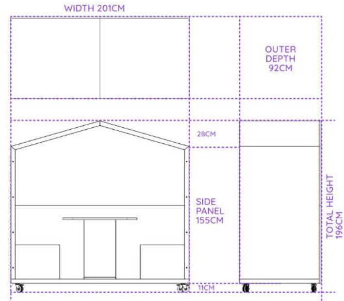
SINGLE NOOK POD DIMENSIONS:
