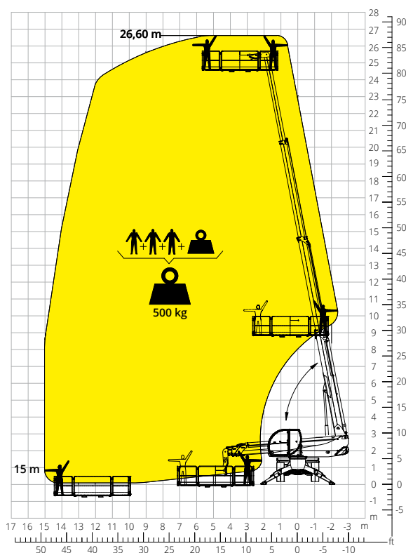
Load chart with ROTATING EXTENDABLE PLATFORM 500 kg ATT - 01 - 005
