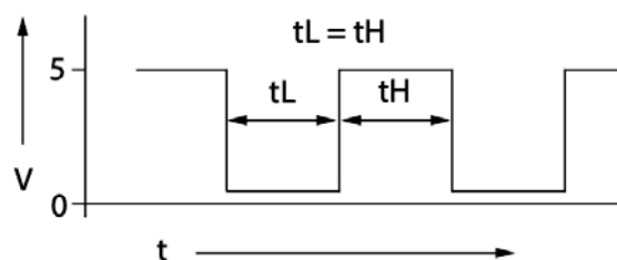
Speed Output Signal
