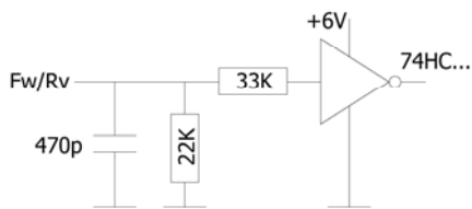
Direction input circuit
