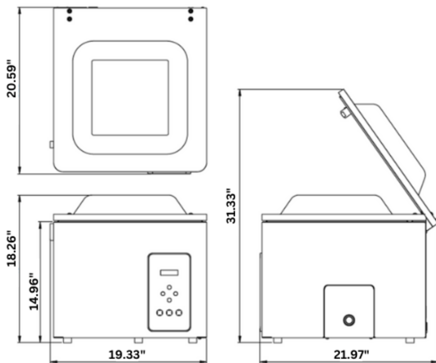
Unit Dimensions
