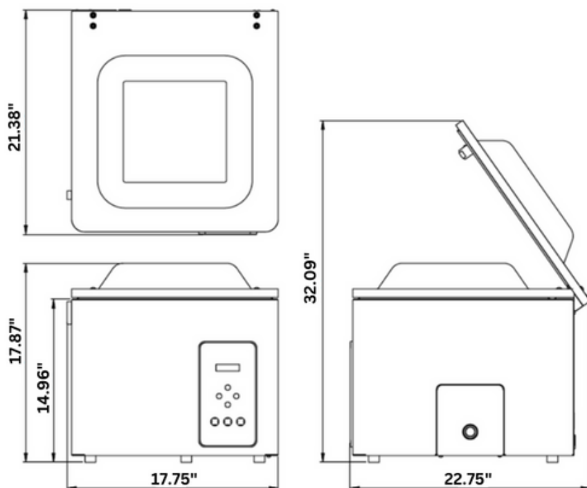
Unit Dimensions
