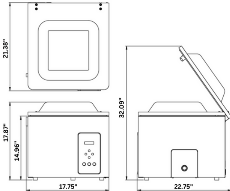
Unit Dimensions
