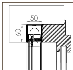
BORA TOP INCAS STANDARD 50/35
