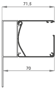
ZCA14Q + ZAC01H
