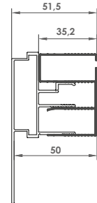
ZCA11Q + ZAG01Q
