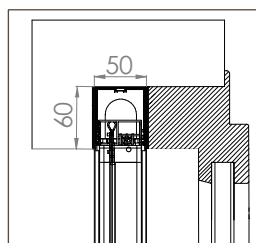
BORA TOP INCAS STANDARD 50/50
