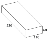
60 Paver 220x110x60mm
