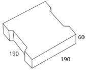
Lock 60 190x190x60mm
