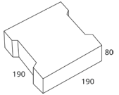
Lock 80 190x190x80mm
