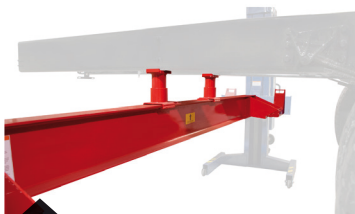
CROSS-BEAM ADAPTER PART # CLHM-CB-32A
