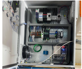
VFD installation and commissioning
