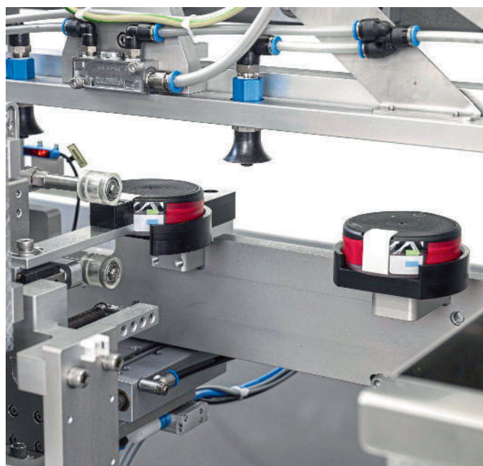
ATD Machinery's ABM60 for an efficient packaging process
