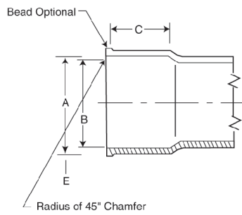
Fittings Socket Dimensions - Inches
