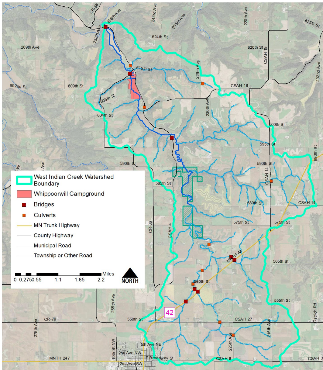
Figure 27. Bridges and culverts that would benefit from upland water retention in the West Indian Creek Watershed
