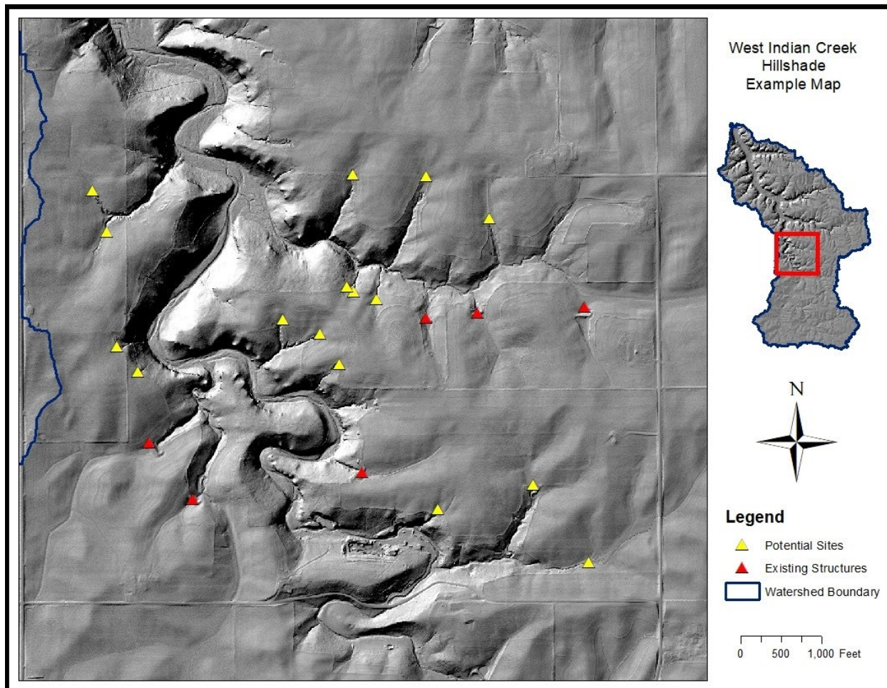
Figure 25. Existing and potential structural BMP sites illustrated with hillshade map
