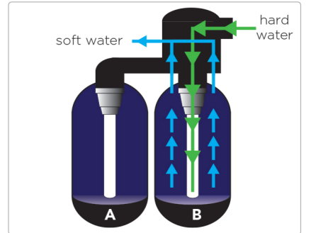
Tank A in stand-by, ready to be used. Tank B is softening the water.
