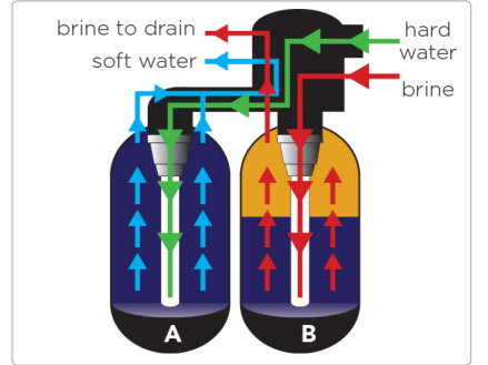
Tank A is softening the water. Tank B is full of limescale minerals and is going through regeneration.
