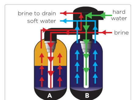
Tank A is full of limescale minerals and is going through regeneration. Tank B is softening the water.
