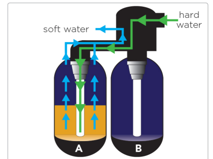
Tank A is softening the water. Tank B in stand-by, ready to be used.
