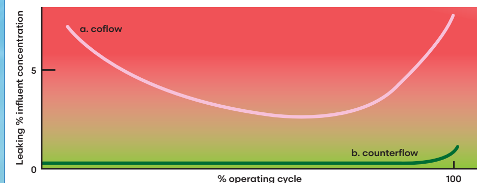
Typical hardness leakage profiles (schematic) during the softening cycle
