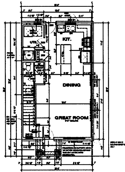
FIRST FLOOR PLAN SCALE 1/8"=1'-0"
