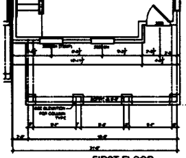
FIRST FLOOR STOCKTON C SCALE 1/8"=1'-0"
