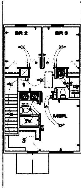
SECOND FLOOR PLAN SCALE 1/8"=1'-0"
