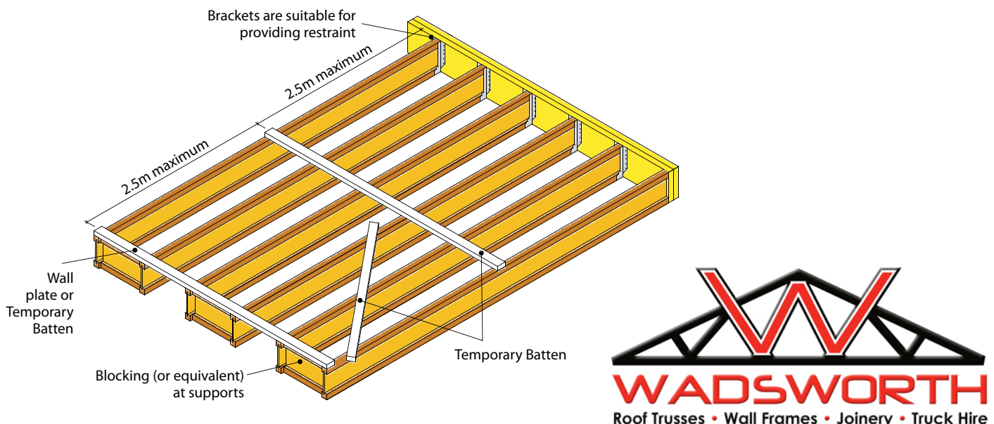
Figure 7: Temporary top flange restraint
