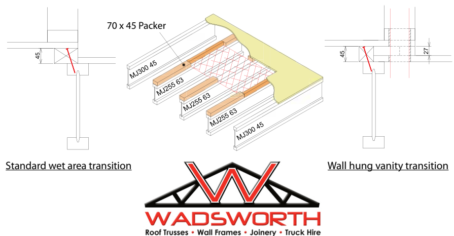
Figure 11: Typical 45mm set down details
