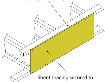
Blocking with sheet bracing
