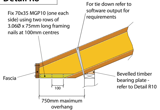
Rafter overhang: horizontal soffit with bevelled plate support
