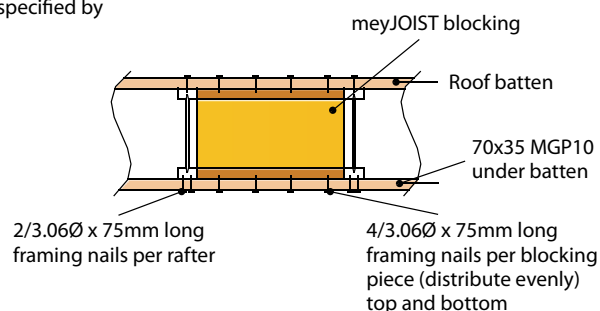
Intermediate lateral restraint for rafters: using battens and blocking
