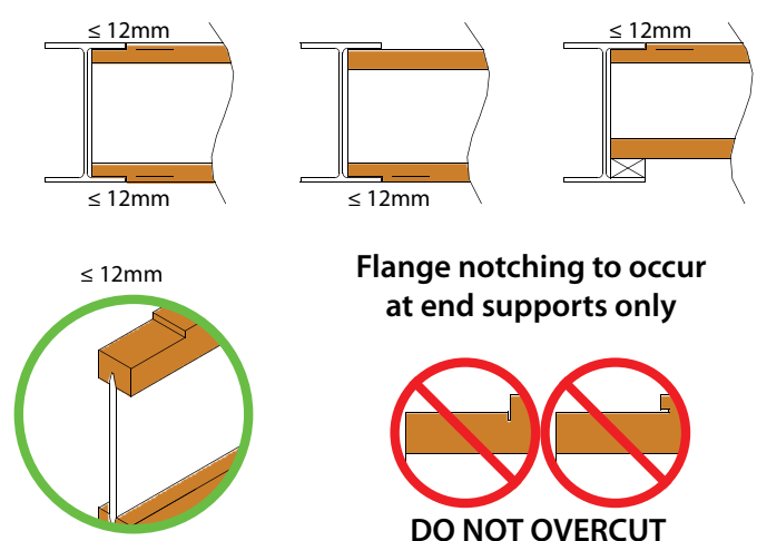
Figure 12: Flange notching
