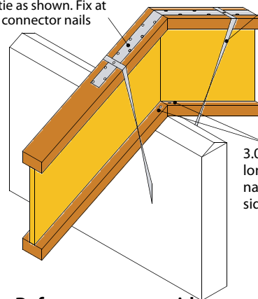
Rafter support at ridge: supported on a bevelled plate
