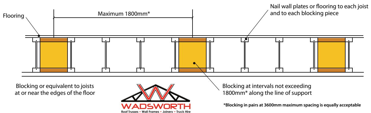
Figure 6: Intermittent Blocking (or Equivalent) at Supports
