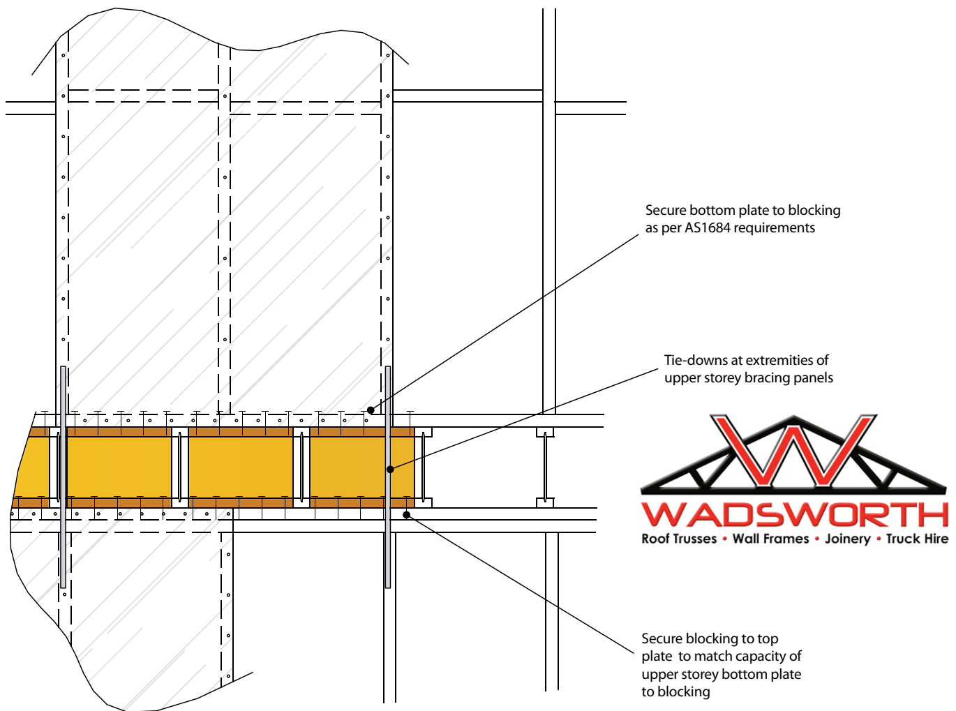
Figure 18: Example of Continuous Blocking and tie-down for high capacity bracing units (eg. > 3.4kN/m)
