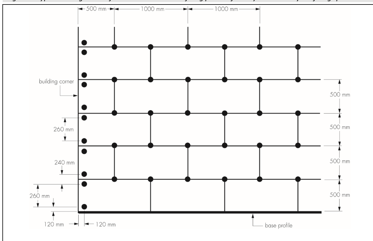
Figure 5 Typical arrangement of insulation boards and fixing pattern for 30-year durability – 2 fixings per board
