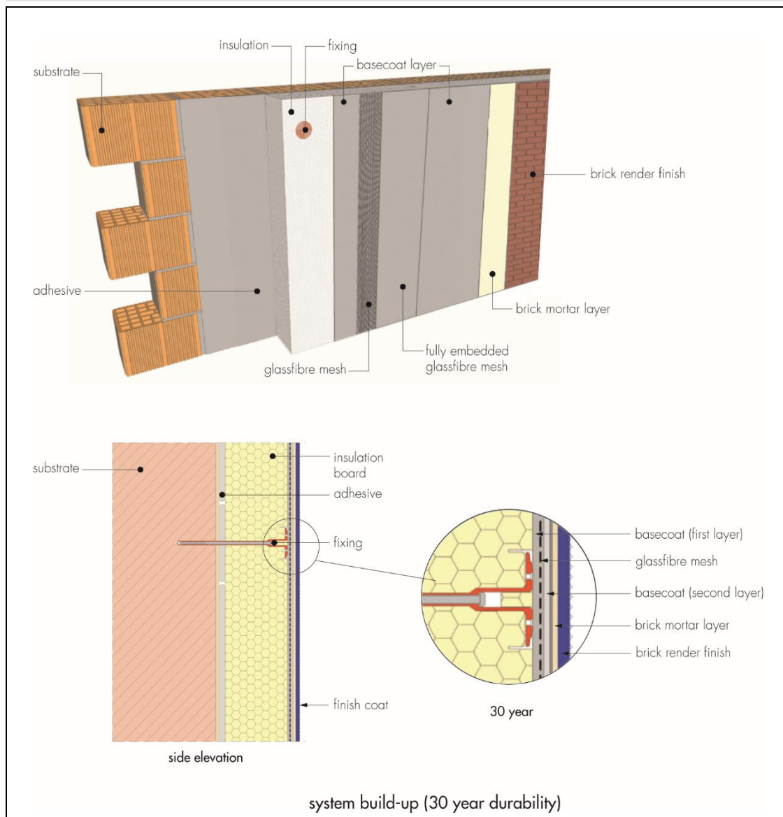
Figure 1a Jubizol EPS Brick Render External Wall Insulation System (30-year durability)
