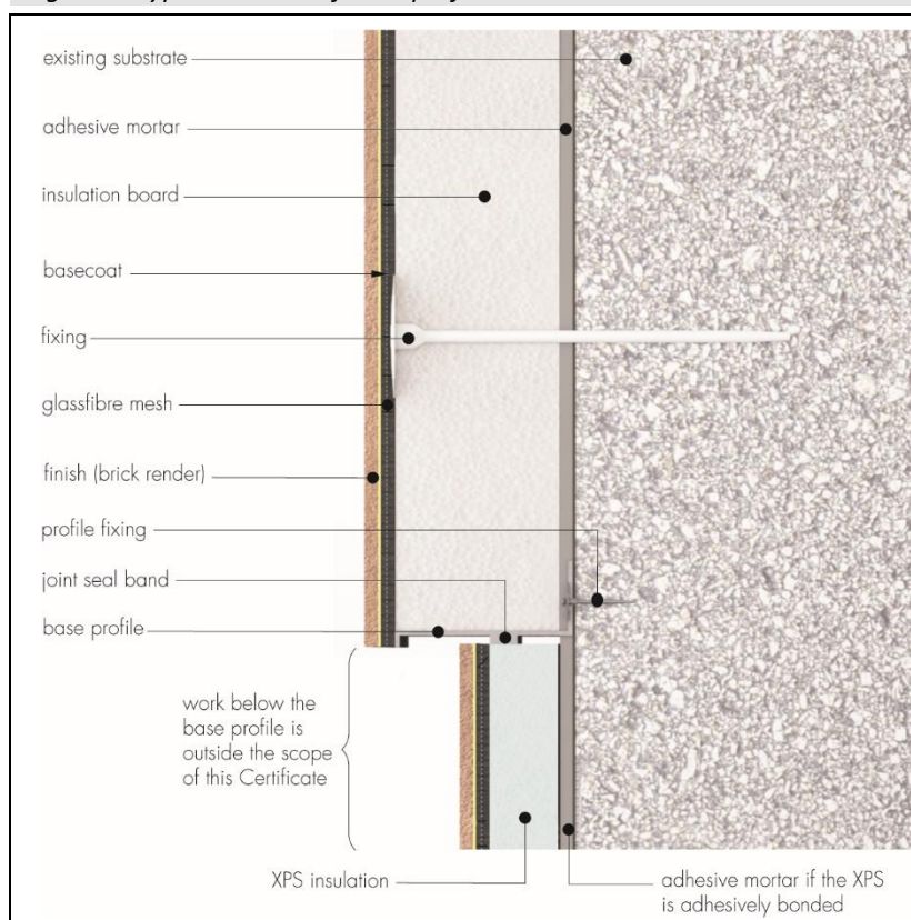
Figure 3 Typical section of base profile
