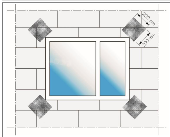
Figure 7 Additional reinforcement of openings
