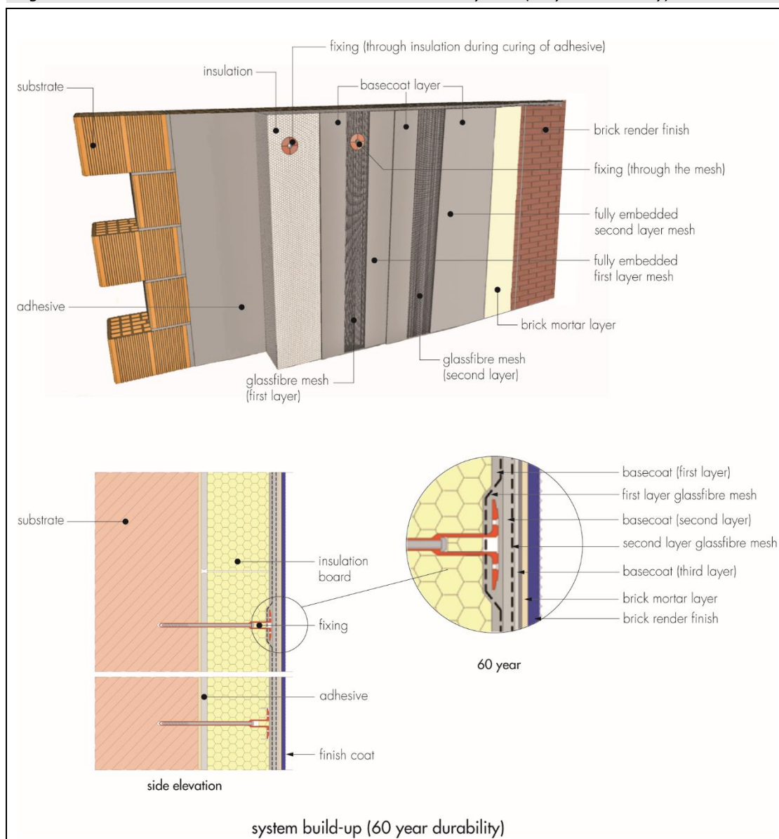
Figure 1b Jubizol EPS Brick Render External Wall Insulation System (60-year durability)
