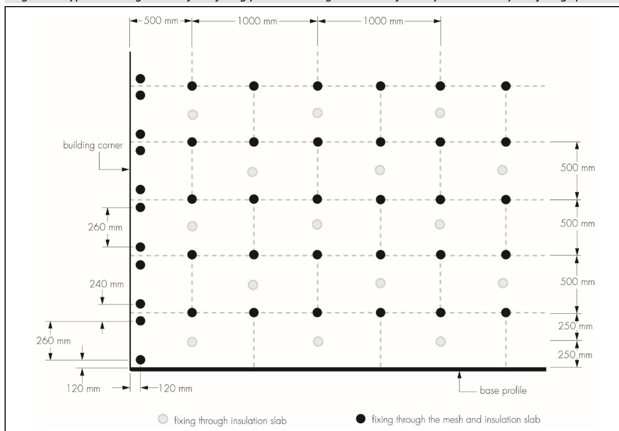
Figure 6 Typical arrangement of the fixing pattern through the mesh for 60-year durability – 6 fixings per m 2
