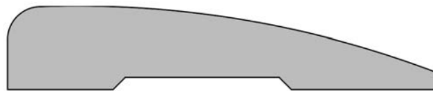
#4042 5/8" x 3 1/4"
