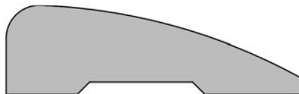
#4041 11/16" x 2 1/4"
