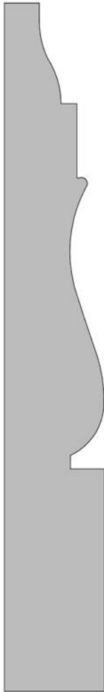
#3021 3/4" x 5 1/4"
