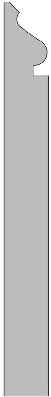
#3025 3/4" x 6 5/8"
