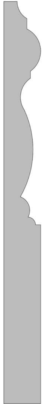
#3010 11/16" x 7 1/4"
