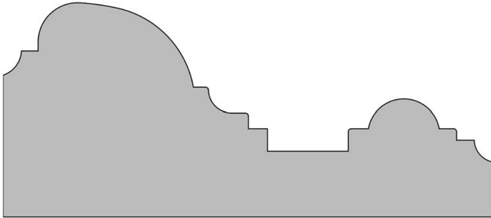
#4034 2 3/16" x 5"
