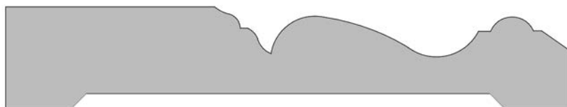
#4013 3/4" x 4 1/4"
