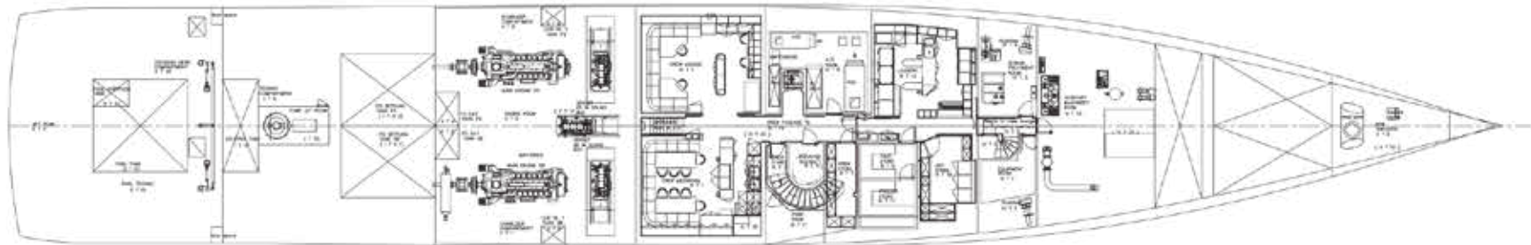
Tank Deck
