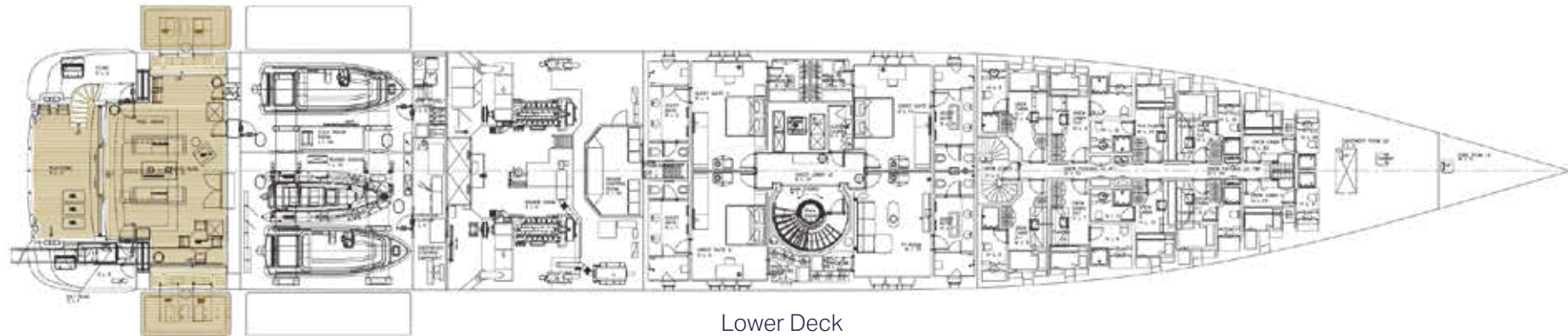
Lower Deck
