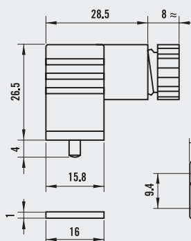
STD Connector
