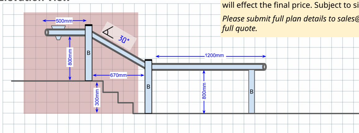
Elevation View
