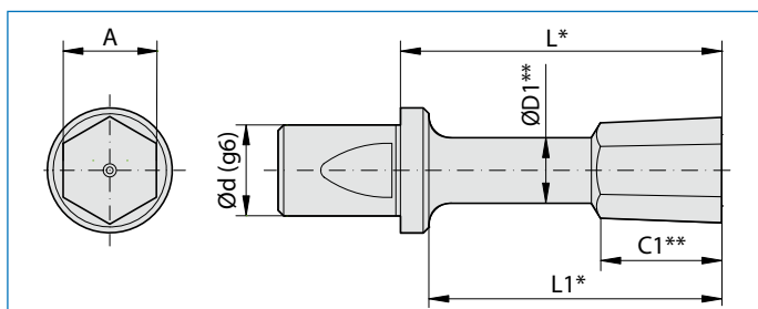
"G8A" - "G8AK" STANDARD "G8A" - "G8AK" STANDARD
