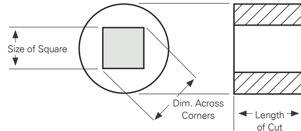
Dimensions of Standard Full Square Broach Holes
