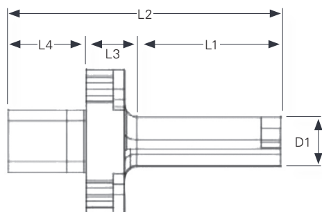
MH 35 / 50 / 65 Square Series Insert Holder
