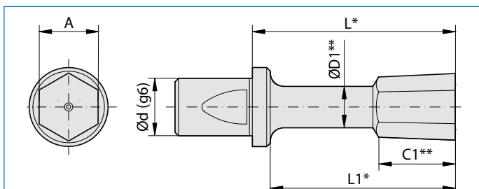
"GP12A" - "GP12AK" STANDARD "GP12A" - "GP12AK" STANDARD
