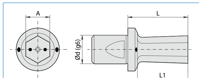
"G12C" - "G12KC" CON PASSAGGIO REFRIGERANTE INTERNO "G12C" - "G12KC" WITH INTERNAL FLOW OF COOLANT
