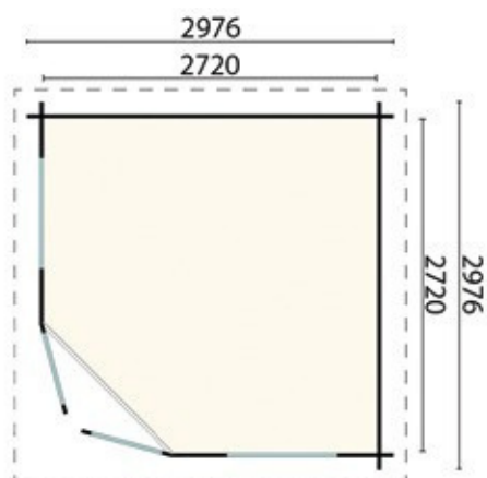
FLAT 280 floor plan
