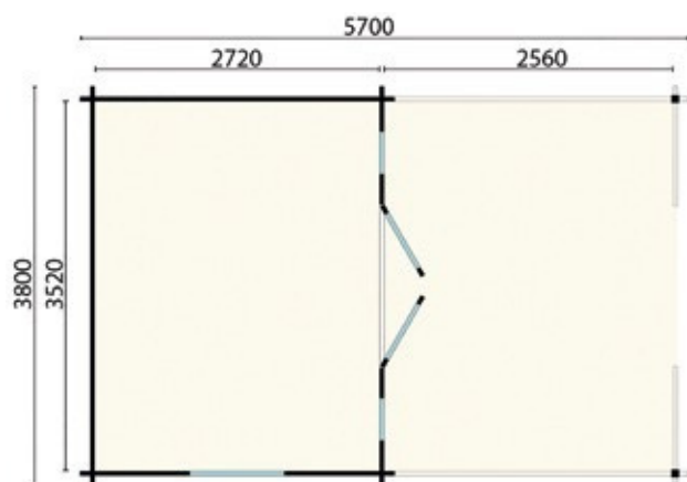
HANNA 1 floor plan
