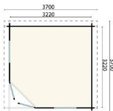
FLAT 330 floor plan
