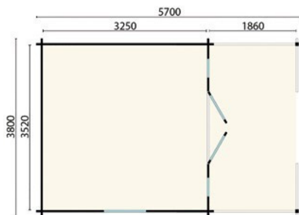
HANNA 2 floor plan
