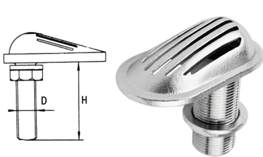
AISI316 STAINLESS STEEL INTAKE STRAINER 316不锈钢海底门
