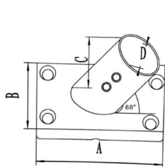
AISI316 STAINLESS STEEL HANDRAIL 60°RECTANGULAR BASE 316不锈钢60° 方管座
