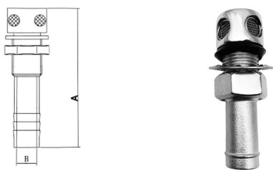
AISI316 STAINLESS STEEL TANK VENT 316不锈钢出气口
