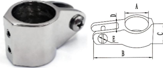
AISI316 STAINLESS STEEL TOP SLIDE 316不锈钢带棱角双顶丝滑套
