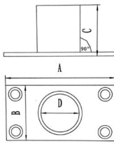
AISI316 STAINLESS STEEL HANDRAIL 90°RECTANGULAR BASE 316不锈钢90° 方管座
