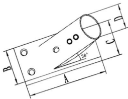
AISI316 STAINLESS STEEL HANDRAIL 30°RECTANGULAR BASE 316不锈钢30° 方管座
