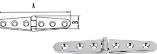
AISI316 STAINLESS STEEL CASTING HINGE 316不锈钢对称合页
