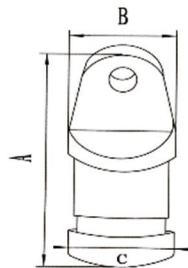
AISI316 STAINLESS STEEL TOP CAP 316不锈钢球形滑帽
