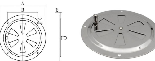
STAINLESS STEEL ROUND AIR LOUVER VENT(SLIDE KHOB OPENING) 316不锈钢圆形百叶风口 (滑动孔)
