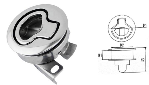
AISI316 STAINLESS STEEL TURNING LOCK 316不锈钢地板锁/护套款
