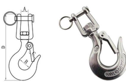
SWIBEL JAW CRANE HOOK 叉式旋转货钩
