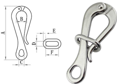
QUICK RELEASE HOOK 释放钩
