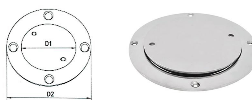
AISI316 STAINLESS STEEL ANTENNA BASE AISI316不锈钢甲板圆盘
