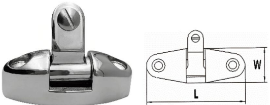
AISI316 STAINLESS STEEL DECK SWIVEL HINGE MOUNT 316不锈钢180° 旋转山型座
