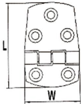
AISI316 STAINLESS STEEL CASTING HINGE 316不锈钢合页
