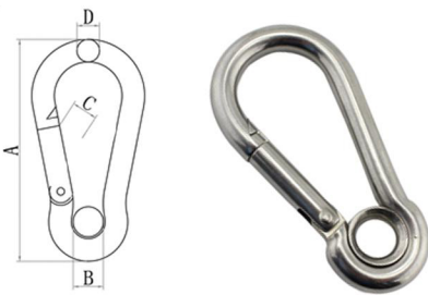
CARABINER HOOK WITH EYELET 带圈登山扣
