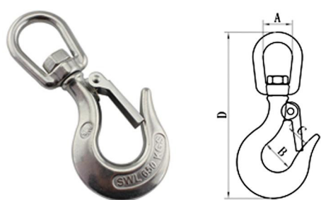
SWIVEL EYE CRANE HOOK 圈式旋转货钩
