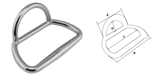
AISI316 STAINLESS STEEL PULL HANDLE LASHING FLUSH D LIFT RING 316不锈钢方拉手捆扎平齐吊环
