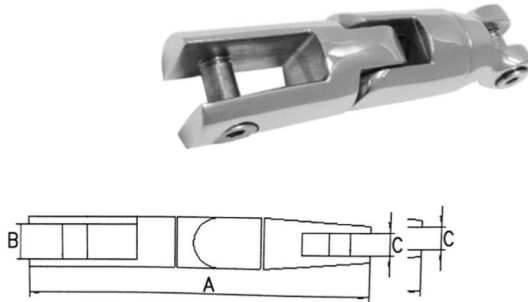
AISI316 STAINLESS STEEL ANCHOR CONNECTOR 316不锈钢长锚连接器
