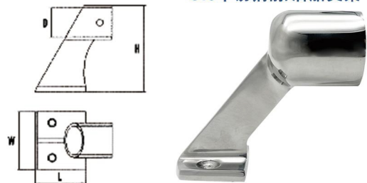
AISI316 STAINLESS STEEL HANDRAIL STANCHION (CENTER 60°) 316不锈钢前/后船支架
