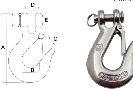
CRANE HOOK WITH LATCH 羊角滑钩
