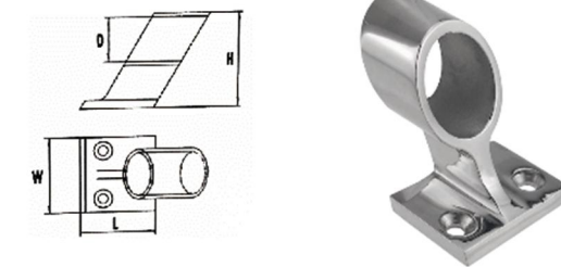
AISI316 STAINLESS STEEL HANDRAIL STANCHION (END 60°) 316不锈钢末尾船支架
