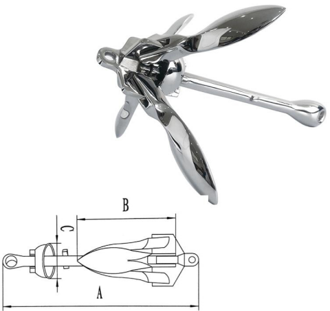
AISI316 STAINLESS STEEL GRAPNEL ANCHOR 316不锈钢伞锚/折叠锚
