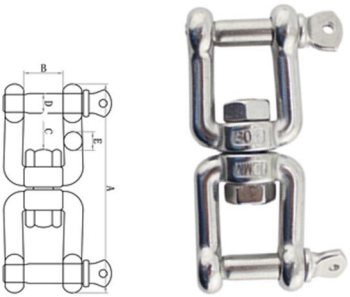
JAW&JAW END SWIVEL 叉叉旋转环
