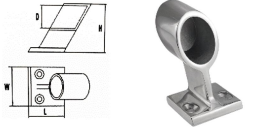
AISI316 STAINLESS STEEL HANDRAIL STANCHION (FORWARD 60°) 316不锈钢前船支架
