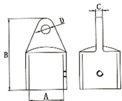
AISI316 STAINLESS STEEL TOP CAP 316不锈钢单顶丝滑帽
