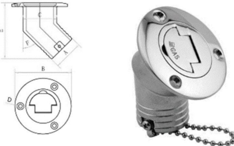
AISI316 STAINLESS STEEL DECK FILLER 316不锈钢弯翻盖油箱体
