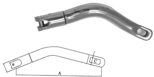
AISI316 STAINLESS STEEL ANCHOR CONNECTOR 316不锈钢长锚连接器
