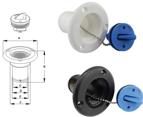
PLASTIC FUEL FILLETR FOR RV 房车加油口
