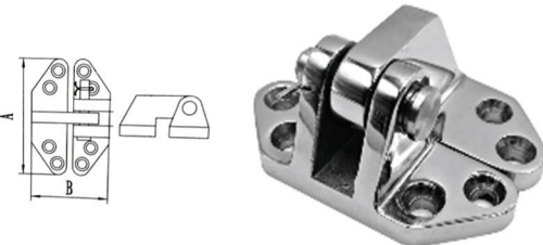
AISI316 STAINLESS STEEL CASTING HATCH HINGE 316不锈钢合页
