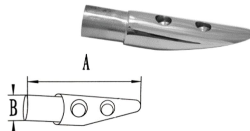
AISI316 STAINLESS STEEL RAIL END 316不锈钢内孔管子支架
