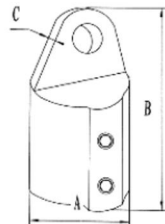
AISI316 STAINLESS STEEL TOP CAP 316不锈钢单顶丝滑帽
