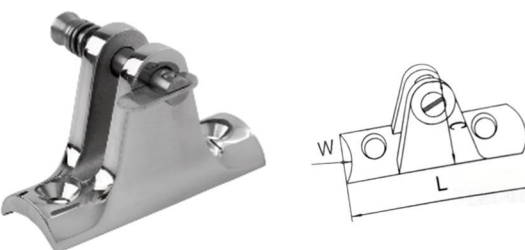
316 STAINLESS STEEL CONCAVE BASE DECK HINGE - REMOVABLE PIN 316不锈钢弧型带销山型座
