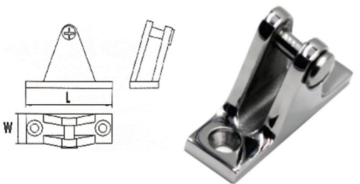
316 STAINLESS STEEL DECK HINGE 60°-REMOVABLE PIN 316不锈钢斜销子山型座
