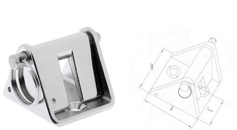
AISI316 STAINLESS STEEL ANCHOR CHAIN STOPPER 316山型止链器
