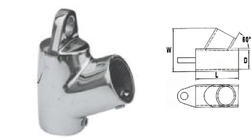
AISI316 STAINLESS STEEL 60° TEE CONNECTOR 316不锈钢60° 提手三通
