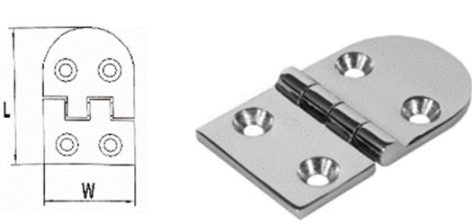
AISI316 STAINLESS STEEL CASTING HINGE 316不锈钢合页
