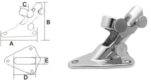
AISI316 STAINLESS STEEL VIBRATION MILLING FLAGPOLE BASE 316不锈钢振动研磨旗杆座
