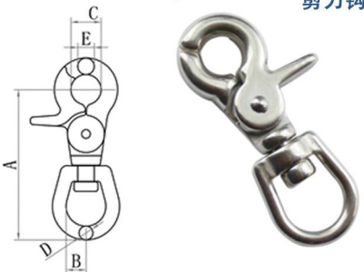
TRIGGER SWIVEL SNAP HOOK 剪刀钩
