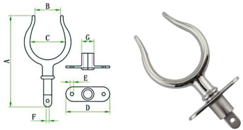
STAINLESS STEEL ROW LOCK 316不锈钢浆叉
