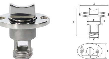
STAINLESS STEEL DIAMOND GARBOARD DRAIN PLUG 316不锈钢子弹头堵头
