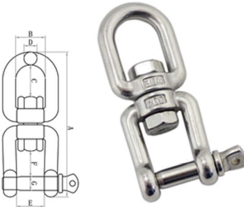
EYE&EYE END SWIVEL 圈叉旋转环
