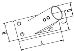
AISI316 STAINLESS STEEL HANDRAIL 45°RECTANGULAR BASE 316不锈钢45° 方管座
