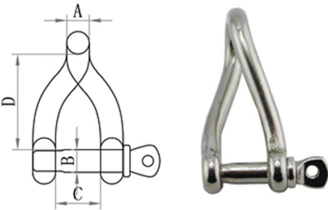
TWISTED SHACKLE 扭体卸扣
