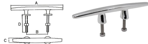
AISI316STAINLESS STEEL HUMPBACKED CLEAT 316不锈钢重驼型索栓
