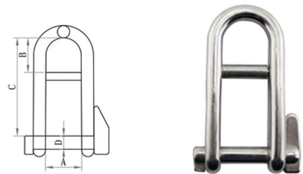
KEY PIN SHACKLE WITH BAR 带档钥匙销卸扣
