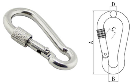
CARABINER HOOK WITH LOCK NUT 带螺母登山扣
