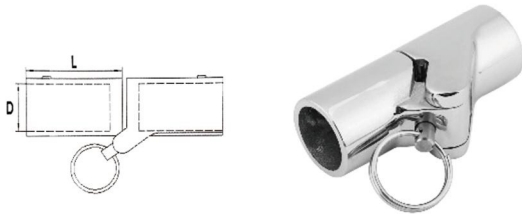
AISI316 STAINLESS STEEL SWIVEL JOINT FOR BIMINI PIPES 316不锈钢拉抽销活节管子接头
