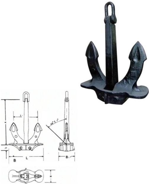
BLACK PAINTED HALL ANCHOR 黑漆霍尔锚
