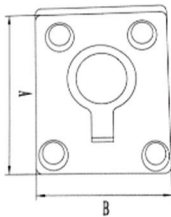
AISI316 STAINLESS STEEL ROUND FLUSH LIFT RING 316不锈钢圆形地板拉环
