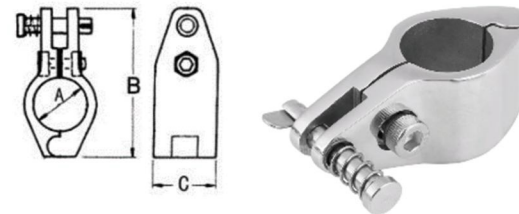
AISI316 STAINLESS STEEL TOP SLIDE WITH PIN 316不锈钢销子管夹
