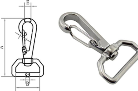
SQUARE SPRING SNAP HOOK 简易方环万向钩
