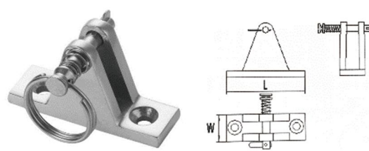
316 STAINLESS STEEL DECK HINGE 90°-REMOVABLE 316不锈钢带环90° 销子山型座
