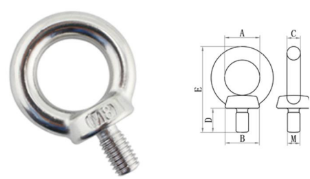
DIN589 EYE SCREW DIN580 吊环螺丝
