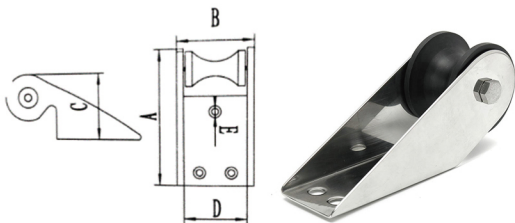
AISI316 STAINLESS STEEL BOW ROLLER 316不锈钢黑色单轮锚支架
