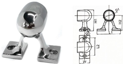
AISI316 STAINLESS STEEL HANDRAIL STANCHION (FORWARD/END 90°) 316不锈钢前/后船支架
