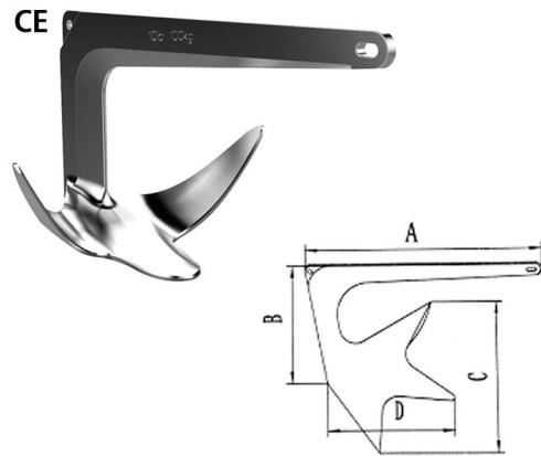
AISI316 STAINLESS STEEL BRUCE ANCHOR 316不锈钢布鲁斯锚
