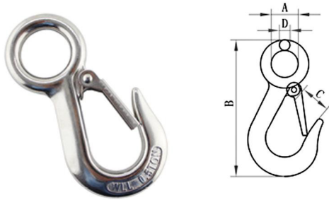
LARGE EYE CRANE HOOK 大眼货钩
