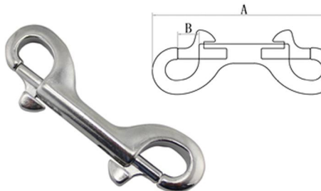
DOUBLE END SNAP HOOK 双头钩
