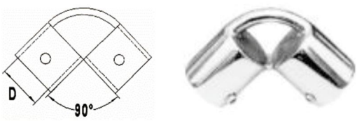
AISI316 STAINLESS STEEL 90°2-WAY TEE CONNECTOR 316不锈钢90°2通三通接头
