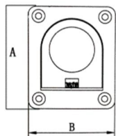
AISI316 STAINLESS STEELSTAMPING SQUARE FLUSH LIFT RING WITH SPRING 316不锈钢冲压地板拉环
