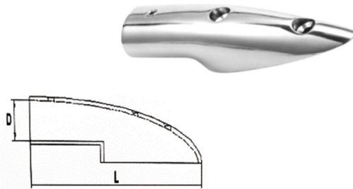
AISI316 STAINLESS STEEL RAIL END 316不锈钢小羊蹄子支架
