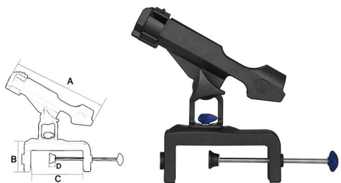
3 COPIES FISHING PLASTIC FISHING ROD HOLDER 可拆卸3联塑料鱼竿座
