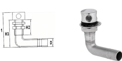
AISI316 STAINLESS STEEL 90 DEGREE TANK VENT 316不锈钢90° 出气口
