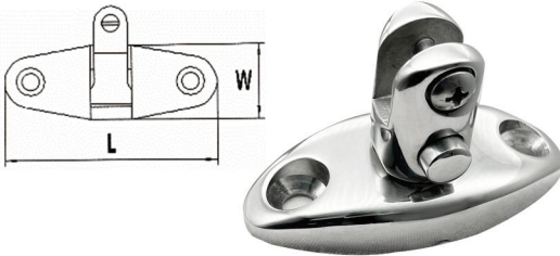
316 STAINLESS STEEL REMOVABLE MOUNTAIN SEAT 316不锈钢可拆卸山型座
