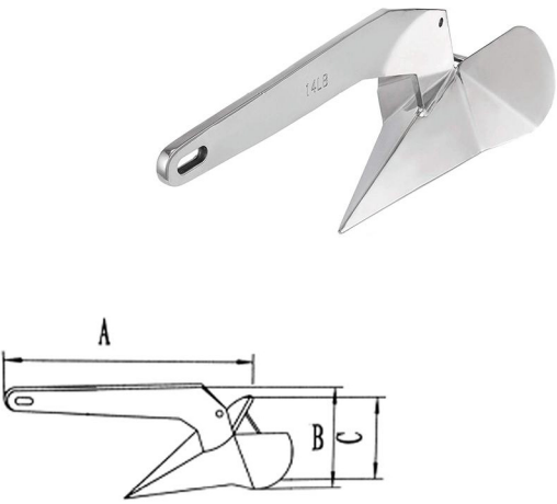
AISI316 STAINLESS STEEL DELTA ANCHOR 316不锈钢三角锚
