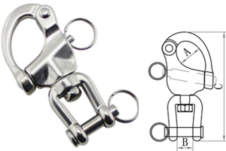
ROUND SWIVEL SNAP SHACKLE 圆环旋转弹簧卸扣
