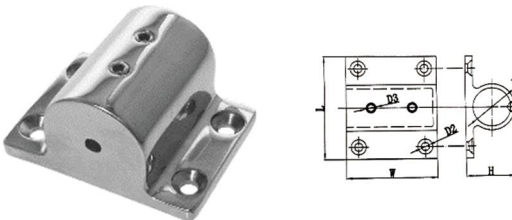
AISI316 STAINLESS STEEL D 316不锈钢方底座支架
