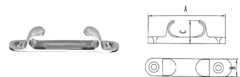
AISI316 STAINLESS STEEL BOW CHOCK 316不锈钢直导缆器
