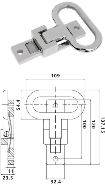
AISI316 STAINLESS STEEL FOLDING STEP 316不锈钢方形马蹄蹬/脚踏
