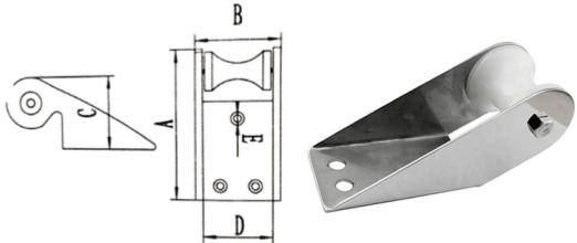
AISI316 STAINLESS STEEL BOW ROLLER 316不锈钢白色单轮锚支架
