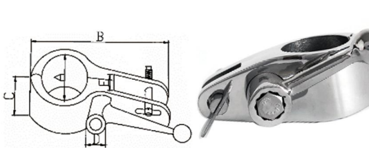
AISI316 STAINLESS STEEL TOP SLIDE 316不锈钢球形把手螺栓管夹
