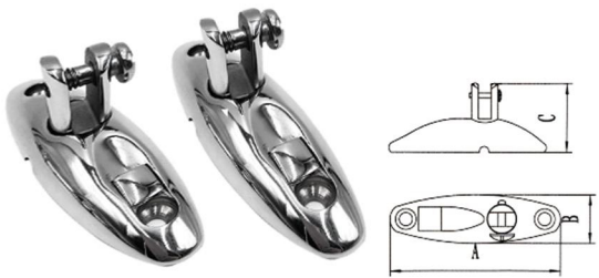
AISI316 STAINLESS STEEL DECK SWIVEL HINGE MOUNT 360° 316不锈钢360° 旋转山型座
