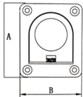
AISI316 STAINLESS STEEL HEAVY SQUARE FLUSH LIFT RING WITH SPRING 316不锈钢重型地板拉环
