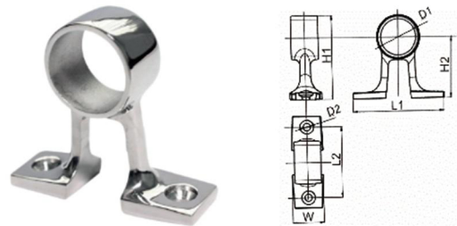
AISI316 STAINLESS STEEL HANDRAIL STANCHION (FORWARD/END 90°) 316不锈钢前/后船支架
