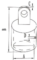
AISI316 STAINLESS STEEL TOP CAP 316不锈钢单顶丝滑帽
