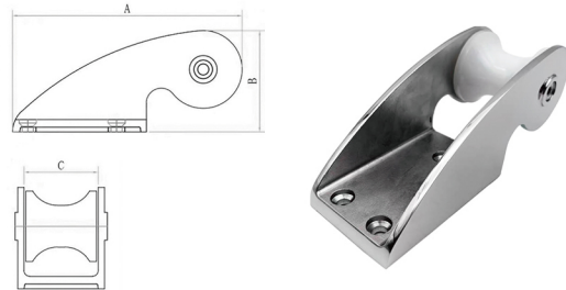
AISI316 STAINLESS STEEL BOW ROLLER 316不锈钢锚支架
