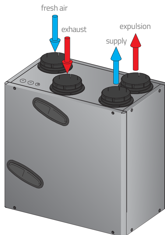
Diagram of the connection of ventilation ducts to the Reversus 200+ HRVU.
