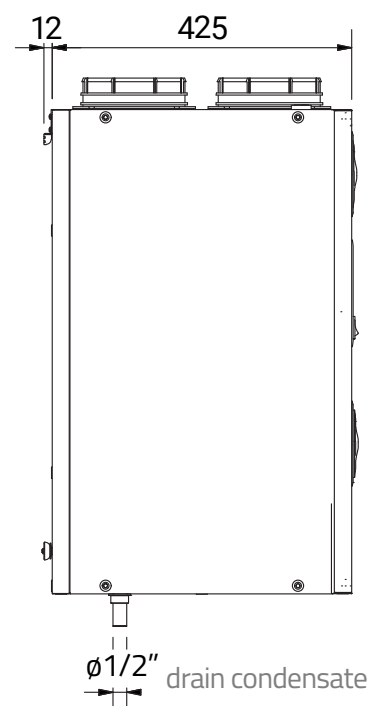
Diagram of the connection of ventilation ducts to the Reversus 200+ HRVU.
