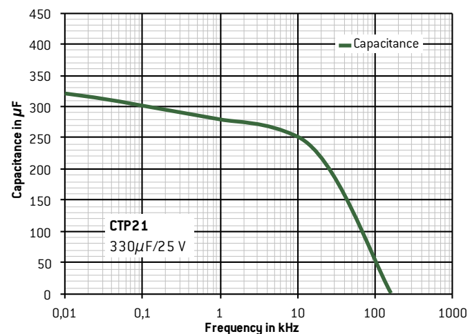
CAPACITANCE CHANGE VS FREQUENCY (TYPICAL)
