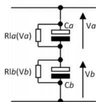
Figure 4 Voltage imbalance
