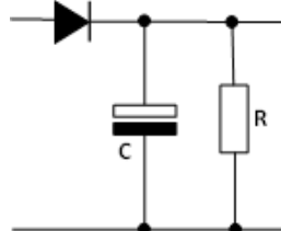
Figure 2 Permanent bleed resistor
