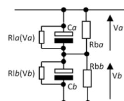
Figure 5 Balancing resistors
