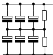
Figure 6 Parallel capacitors
