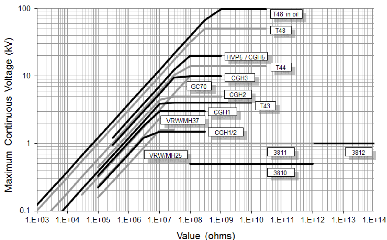
Maximum Voltage Plots for Selected Products
