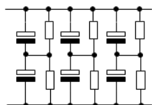
Figure 7 High reliability balancing of parallel capacitors
