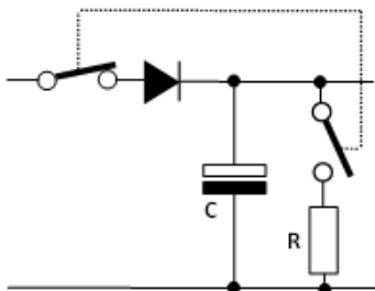
Figure 1 Switched bleed resistor
