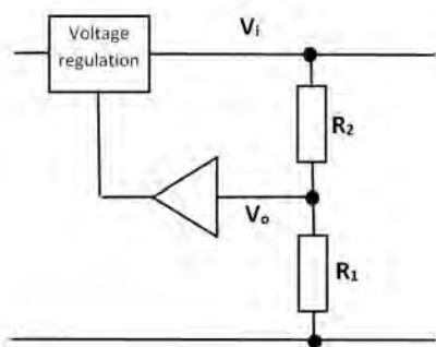
Figure 8 Voltage Divider
