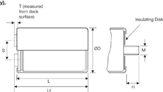
Clamp Mounting
