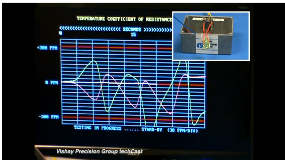
Video 2: Bulk Metal® Foil Resistor TCR Performance
