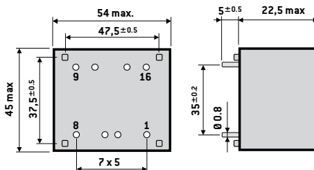
Casing E
