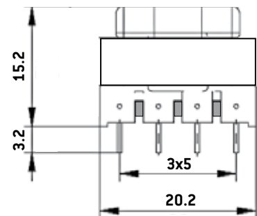
Casing C
