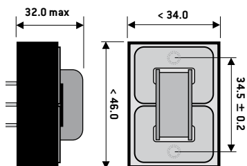
Casing D
