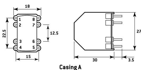
Casing A
