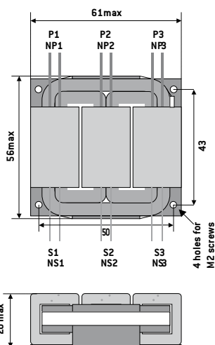
Casing F
