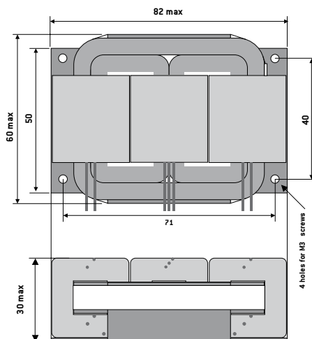
Casing G
