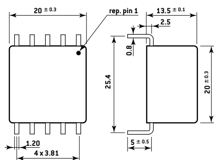
Casing C
