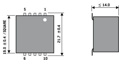
Casing A
