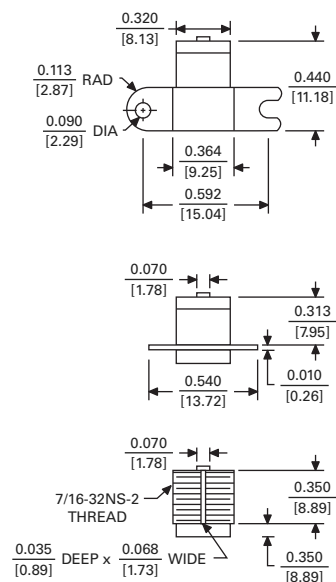
AT104-01, 10AT17-03-10, 10AT15-03-10
