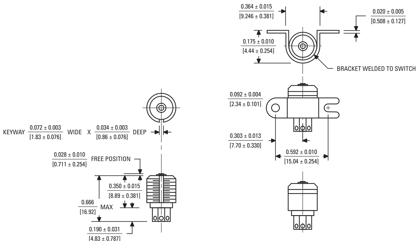
DIMENSIONAL DRAWINGS – Threaded Mount (10AT17-01), Basic Switch (10AT117-01), Bracket Mount (10AT15-01), Flat Plunger
