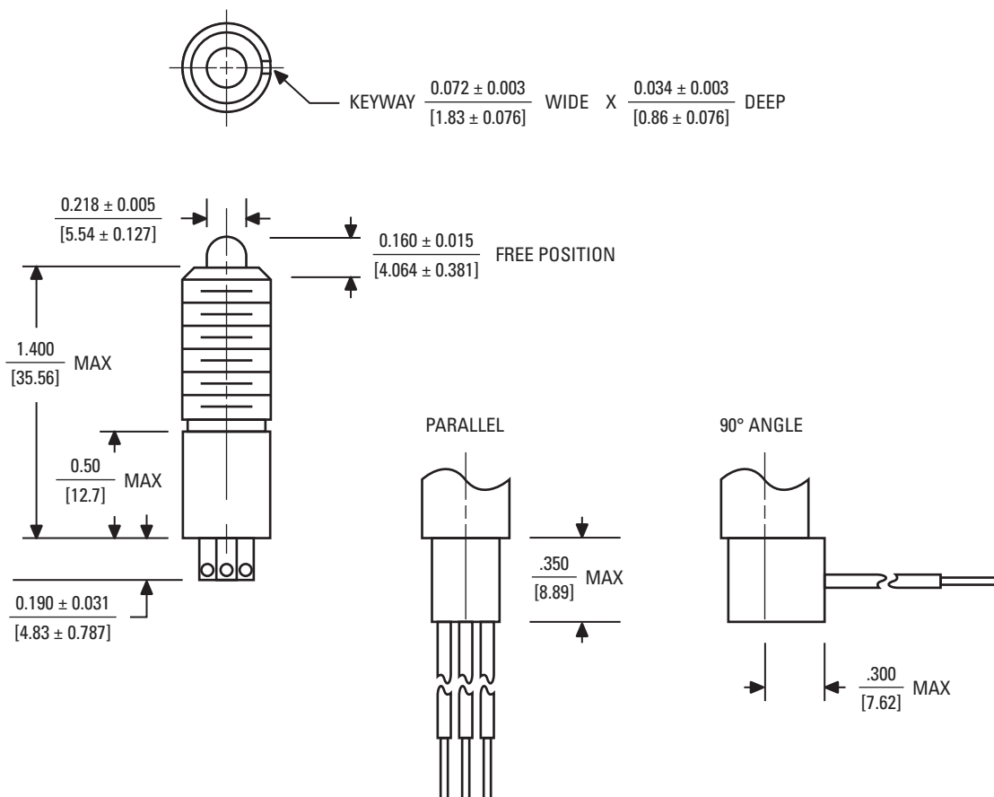
DIMENSIONAL DRAWINGS – Threaded Mount, Spherical Plunger Configuration (10AT367-01, 10AT367-02, 10AT367-03)
