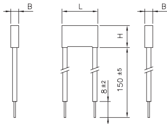
Insulated flexible leads 0.5mm²
