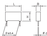
Insulated rigid leads
