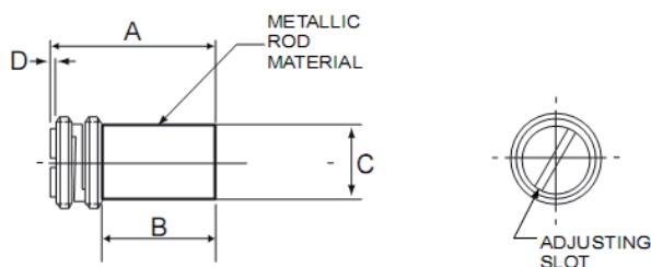
Models made of brass and dimensions in mm
