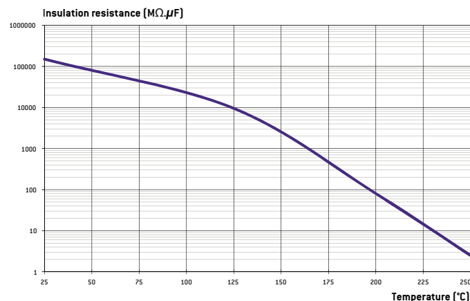
NPO: TYPICAL INSULATION RESISTANCE VERSUS TEMPERATURE
