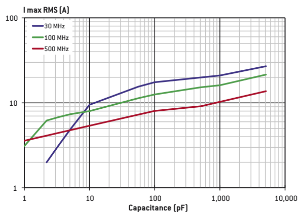
4040: TYPICAL CURRENT RATING VERSUS CAPACITANCE
