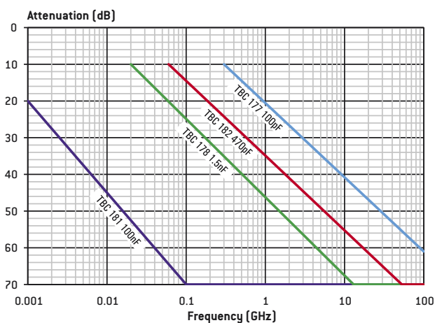
NPO: TYPICAL ATTENUATION CURVE VERSUS FREQUENCY (50 \Omega IMPEDANCE)
