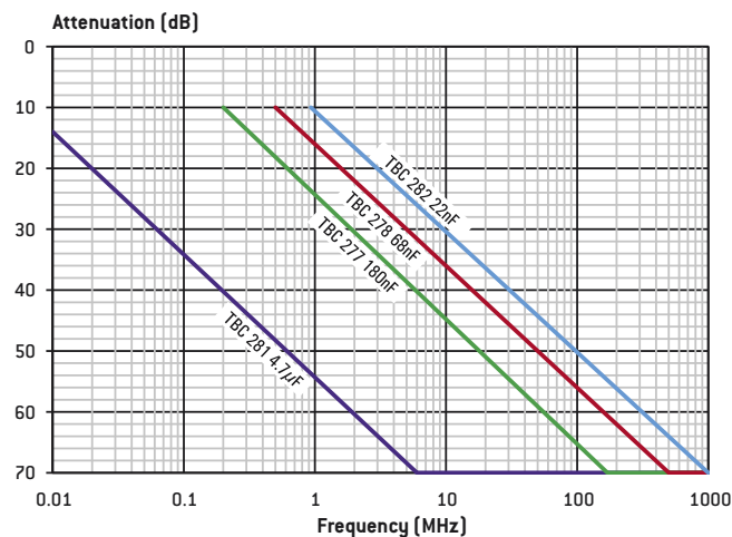
X7R: TYPICAL ATTENUATION CURVE VERSUS FREQUENCY (50 \Omega IMPEDANCE)
