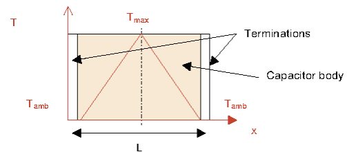
Temperature profile inside the capacitor
