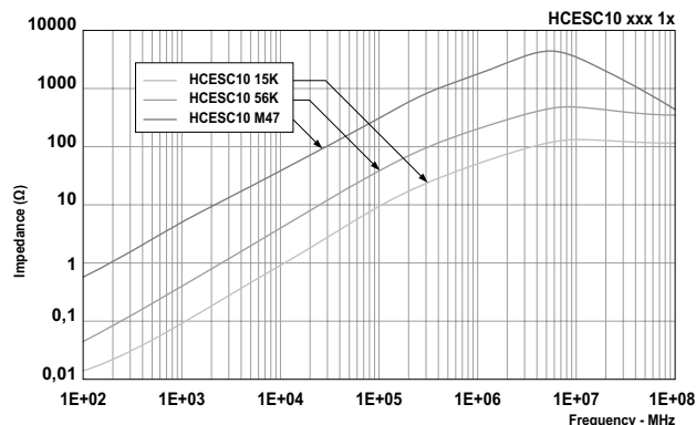
Typical Impedance versus Frequency (@100mV)
