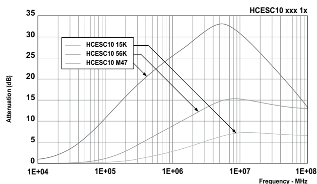
Typical Attenuation versus Frequency on 50 Ohms (@100mV)
