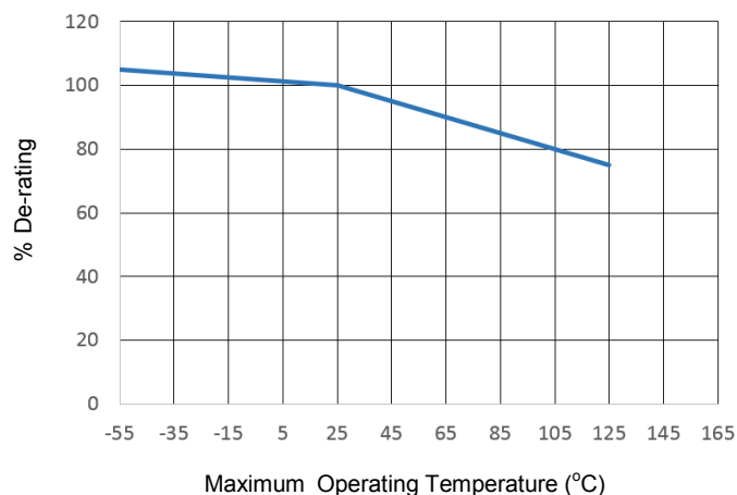
Effect of Ambient Temperature on Current Rating of QA Series
