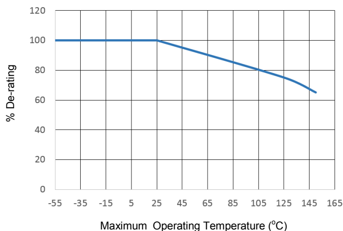
Effect of Ambient Temperature on Current Rating of QF Series
