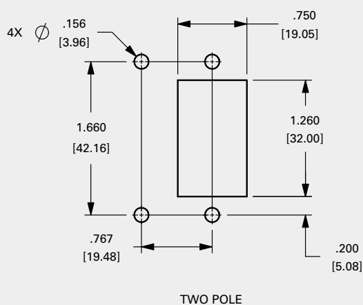
Two Pole, Rocker Handle
