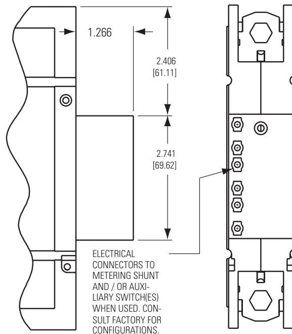
Metering Shunt
