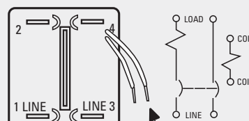
Two Pole (1 pole relay)
