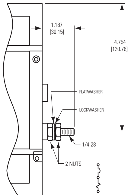
Shunt Trip
