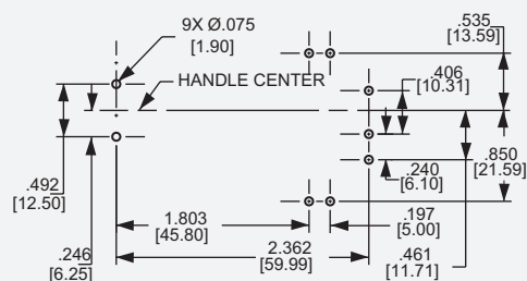
Mounting Detail
