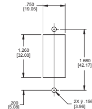
Panel Mounting Detail* Single, Two & Three Pole
