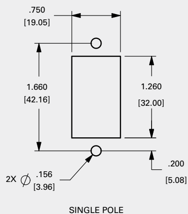
Single Pole, Rocker Handle
