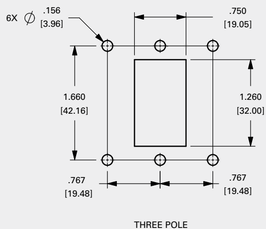
Three Pole, Rocker Handle
