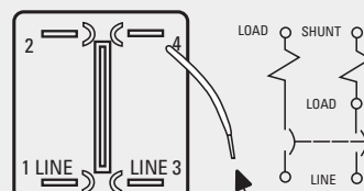
Two Pole ( 1 pole shunt)
