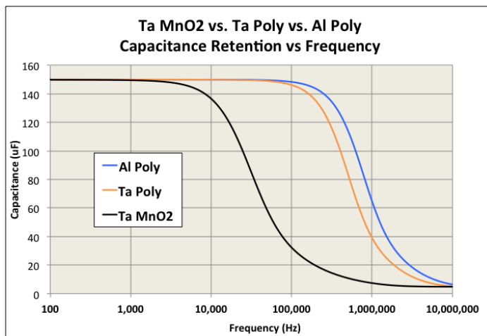
Capacitance vs Frequency: 150 \mu F/6.3V Capacitor
