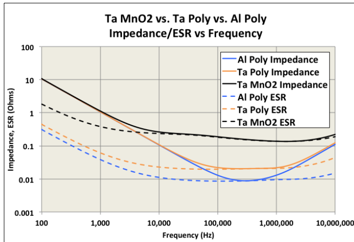
Impedance & ESR Comparison: 150 \mu F/6.3V Capacitor
