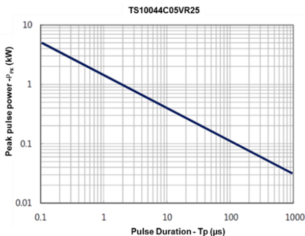
Fig. 4 Non-repetitive peak pulse power vs. Pulse time
