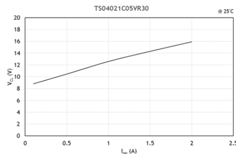
Fig. 6 Clamping voltage ( V_{CL} ) as a function of peak current ( I_{PP} ); t_p = 8/20\mu s
