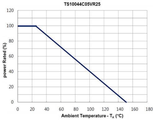
Fig. 5 Power derating vs. Ambient temperature
