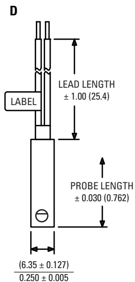
FLANGE MOUNT PROBE 300 STAINLESS STEEL #22 AWG STRANDED, XLPE INSULATED
