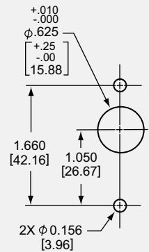
Single Pole Mounting Detail
