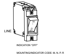
MARKING DETAIL "C" (SEE TABLE)
