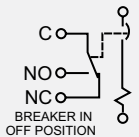
Series with Auxiliary Switch
