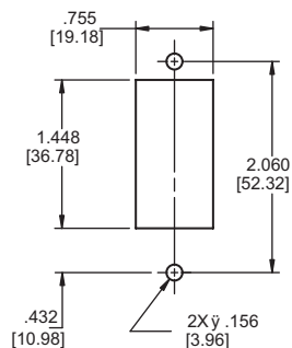
Mounting Detail
