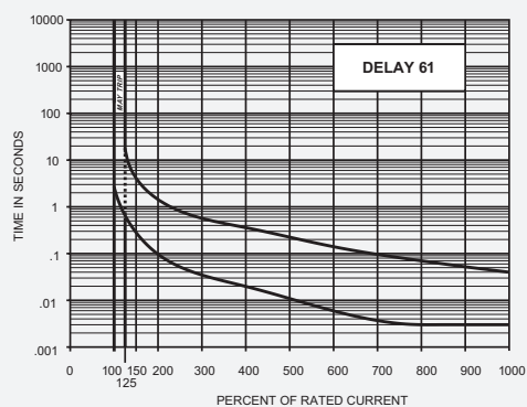
50/60Hz Delay Curves (typ)
