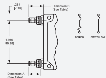
Series and Switch Only
