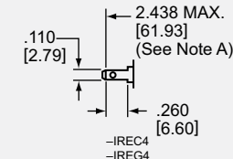
Series with Auxiliary Switch
