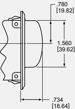
Optional Handle Guard
