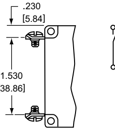
LEG Type Units Require Screw Terminals
