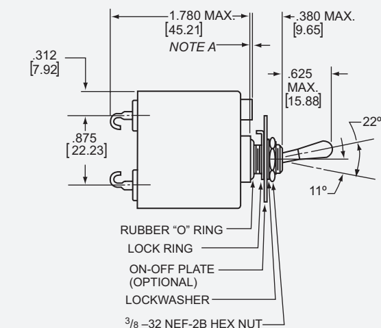
Three Pole, AP112, Toggle
