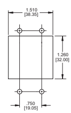
Four Pole**
