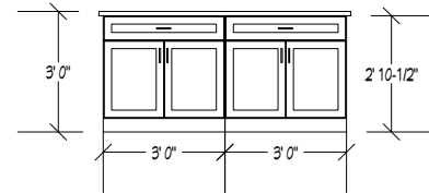
APARTMENT 5 - KITCHEN ISLAND ELEVATION
