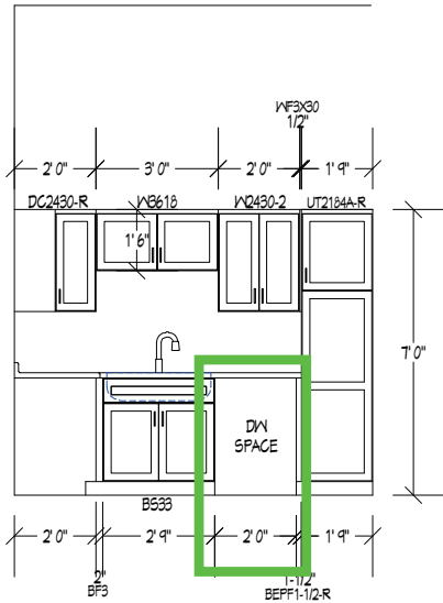
APARTMENT 5 - NORTH KITCHEN ELEVATION
