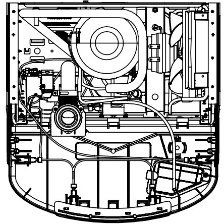
Competitor's Water Cooler 60+ Parts
